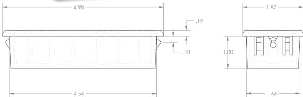
LOUVER 336: RECTANGULAR HOSE ADAPTER: OPTIONAL HOT STAMP: YES METALIZED: NO
