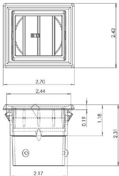
LOUVER 364: SQUARE HOSE ADAPTER: OPTIONAL HOT STAMP: OPTIONAL METALIZED: NO
