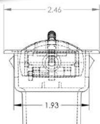
LOUVER 500: RECTANGULAR HOSE ADAPTER: OPTIONAL HOT STAMP: NO METALIZED: NO
