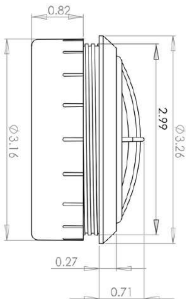
LOUVER 170:ROUND HOSE ADAPTER:OPTIONAL HOT STAMP:NO METALIZED:OPTIONAL
