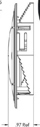
LOUVER 585: ROUND HOSE ADAPTER: NO HOT STAMP: NO METALIZED: NO
