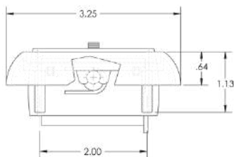
LOUVER 367: RECTANGULAR HOSE ADAPTER: NO HOT STAMP: OPTIONAL METALIZED: NO
