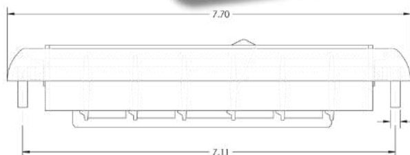
LOUVER 367: RECTANGULAR HOSE ADAPTER: NO HOT STAMP: OPTIONAL METALIZED: NO
