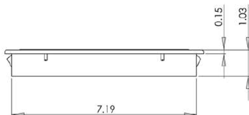
LOUVER 533: RECTANGULAR HOSE ADAPTER: NO HOT STAMP: NO METALIZED: NO
