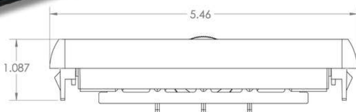
LOUVER 124: RECTANGULAR HOSE ADAPTER: 2.5 " , 2 " HOT STAMP: OPTIONAL METALIZED: NO
