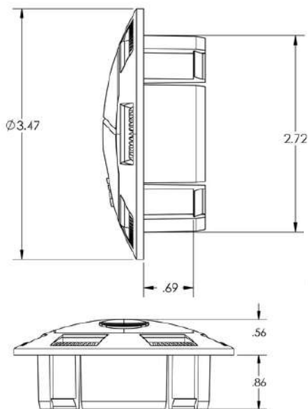
LOUVER 888: ROUND HOSE ADAPTER: OPTIONAL HOT STAMP: NO METALIZED: NO
