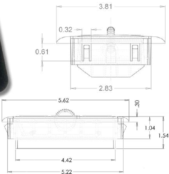
LOUVER 634: RECTANGULAR HOSE ADAPTER: OPTIONAL HOT STAMP: NO METALIZED: NO
