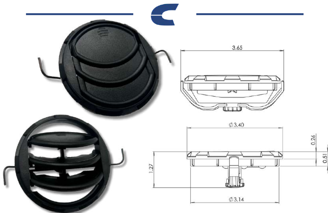
LOUVER 552:ROUND HOSE ADAPTER:NO HOT STAMP:NO METALIZED:NO
