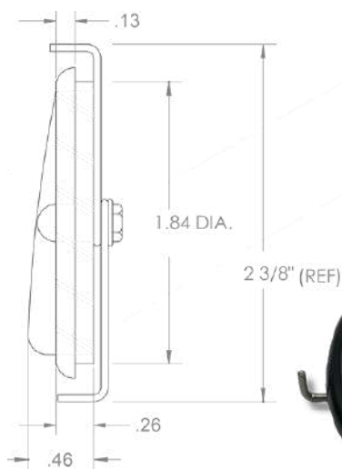
LOUVER 421:ROUND HOSE ADAPTER:NO HOT STAMP:NO METALIZED:NO
