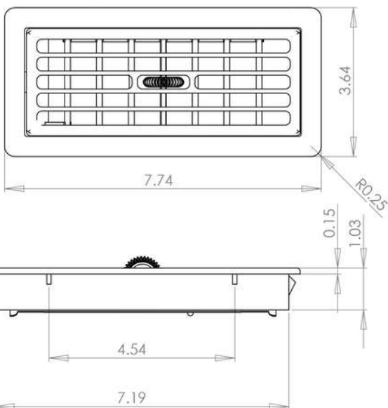
LOUVER 633: RECTANGULAR HOSE ADAPTER: OPTIONAL HOT STAMP: NO METALIZED: NO
