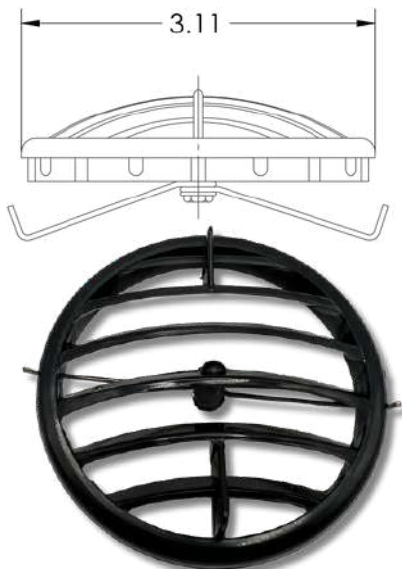
LOUVER 422:ROUND HOSE ADAPTER:NO HOT STAMP:NO METALIZED:NO
