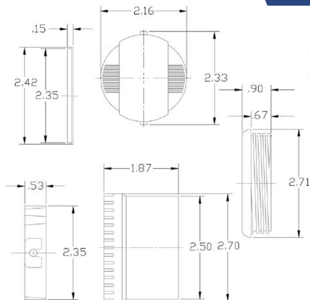
LOUVER 577: BALL/ROUND HOSE ADAPTER: OPTIONAL HOT STAMP: OPTIONAL METALIZED: OPTIONAL
