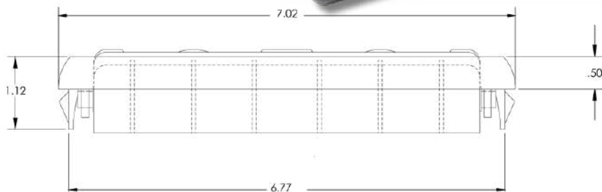
LOUVER 152: RECTANGULAR HOT STAMP: OPTIONAL METALIZED: OPTIONAL
