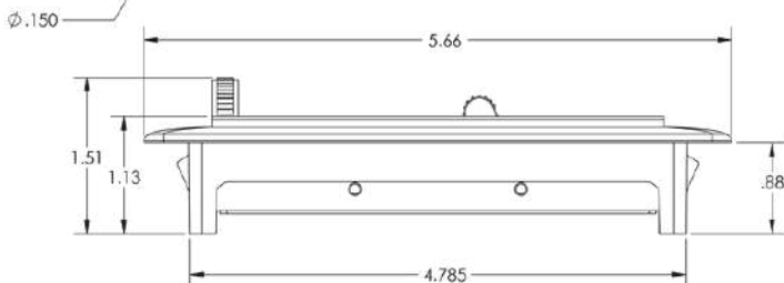
LOUVER 660: RECTANGULAR HOSE ADAPTER: OPTIONAL HOT STAMP: NO METALIZED: NO
