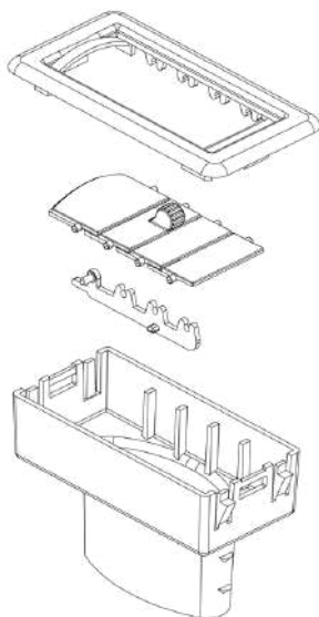
LOUVER 360: RECTANGULAR HOSE ADAPTER: OPTIONAL HOT STAMP: NO METALIZED: NO
