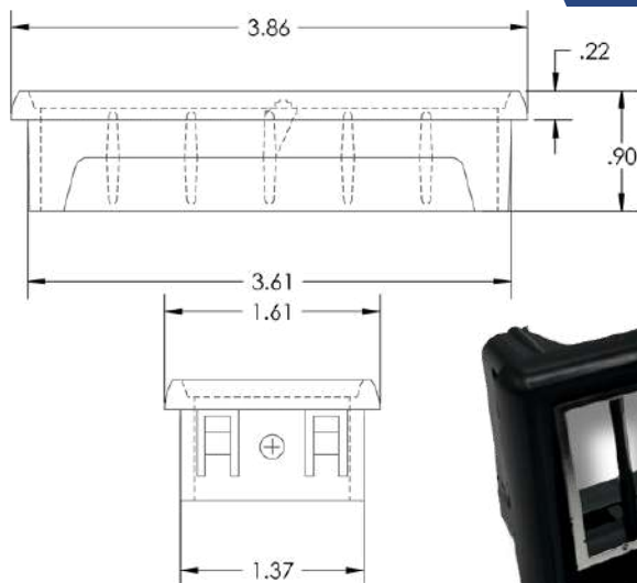
LOUVER 796: RECTANGULAR HOSE ADAPTER: NO HOT STAMP: YES METALIZED: NO
