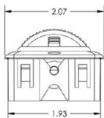
LOUVER 660: RECTANGULAR HOSE ADAPTER: OPTIONAL HOT STAMP: NO METALIZED: NO
