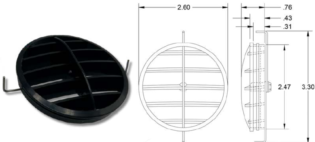
LOUVER 873:ROUND HOSE ADAPTER:NO HOT STAMP:NO METALIZED:NO
