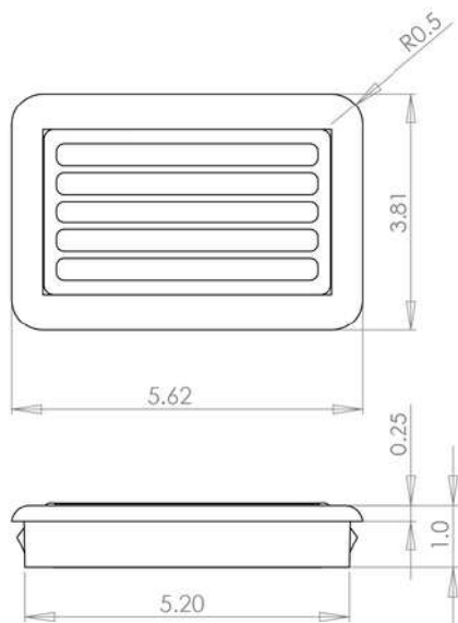
LOUVER 544:RECTANGULAR HOSE ADAPTER:NO HOT STAMP:NO METALIZED:NO
