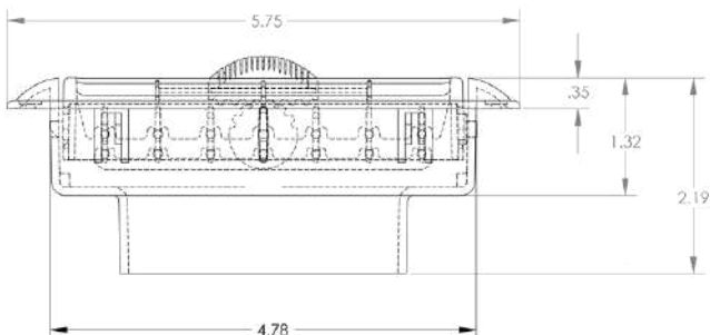
LOUVER 500: RECTANGULAR HOSE ADAPTER: OPTIONAL HOT STAMP: NO METALIZED: NO
